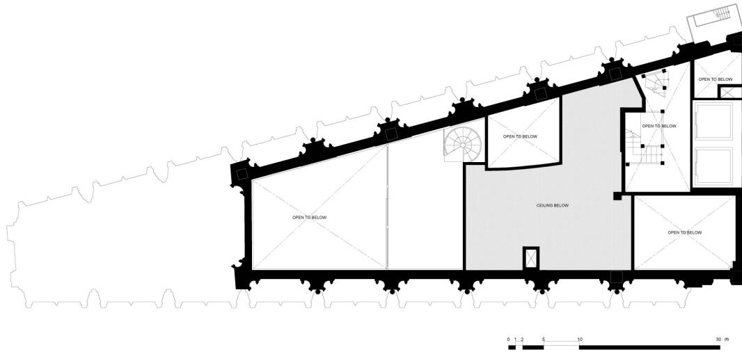
12th Floor Plan-MEZZANINE
