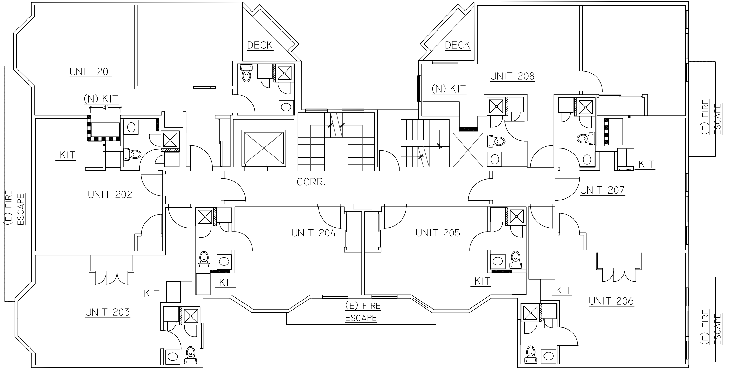
2ND FLOOR PLAN
