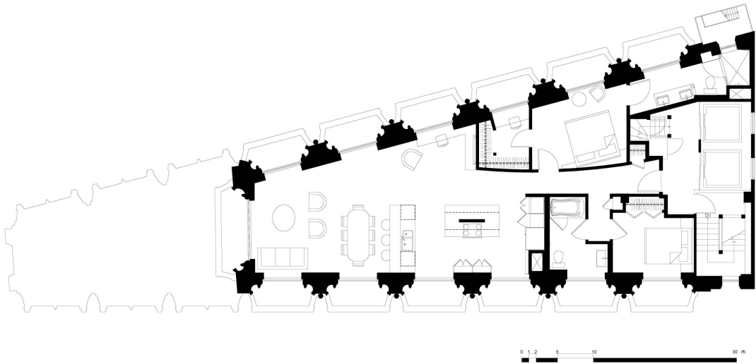
11th Floor Plan
