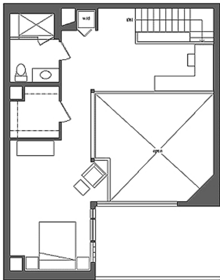
Mezzanine
